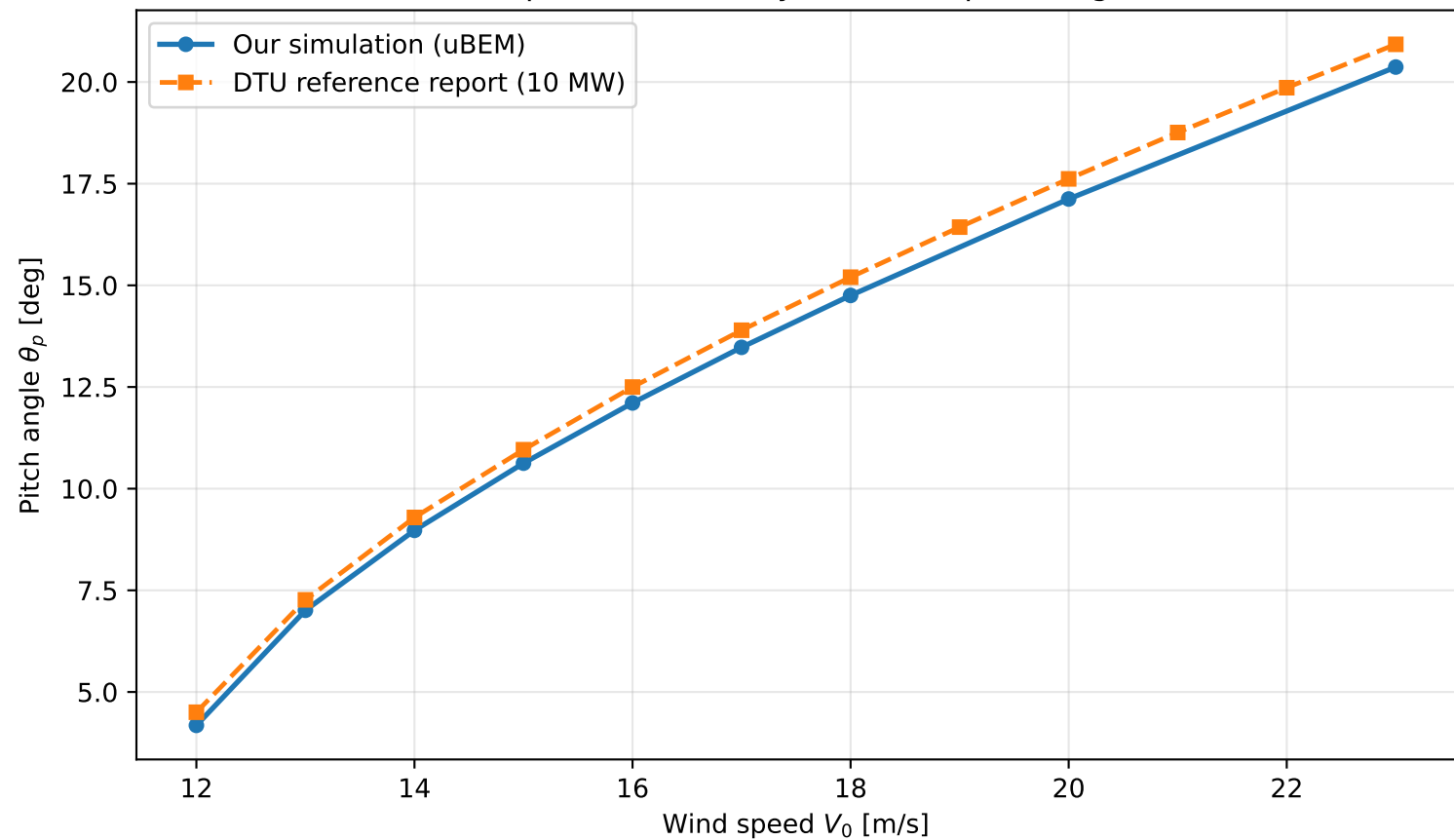
Comparison of steady collective pitch angle
